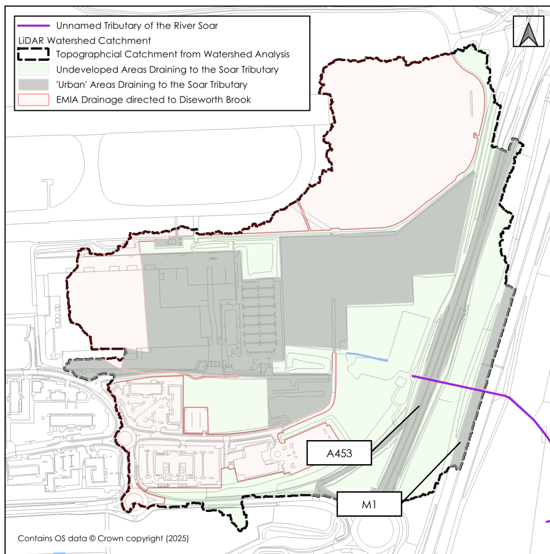
Figure 4 – Watershed Analysis & Measured Urban Areas
